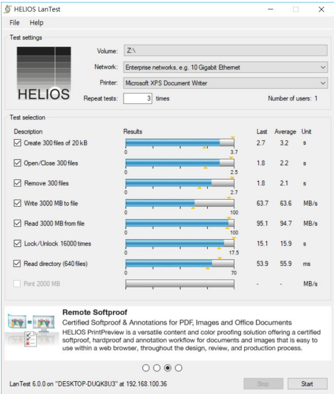
Figure 4 – HELIOS LanTest Before Encryption
