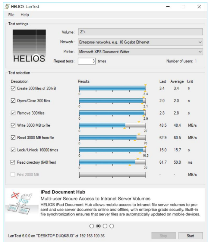
Figure 7 – HELIOS LanTest After Encryption
