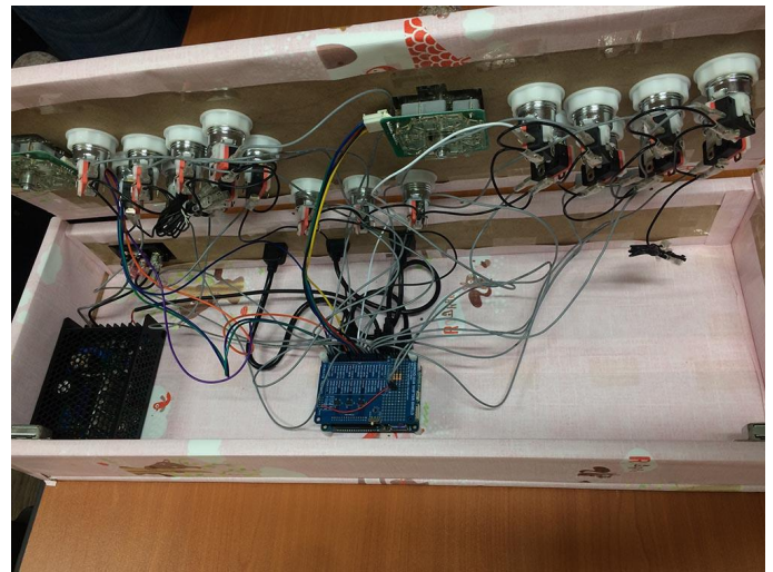
Figure 8 - ODROID Arcade Box Wiring
