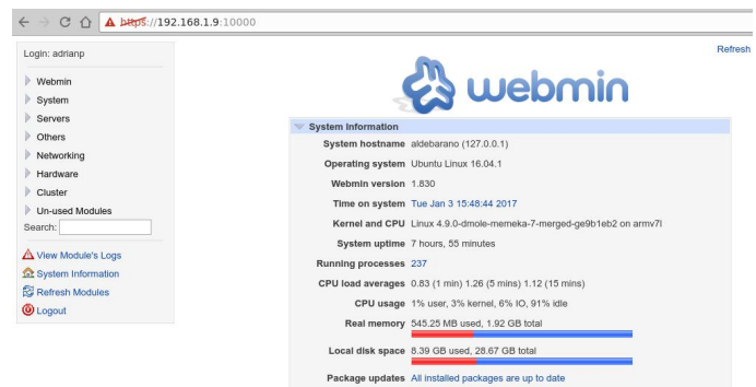
Figure 1 – Stock Webmin interface
