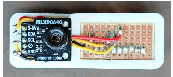
Figure 2 : A photo of the circuit
