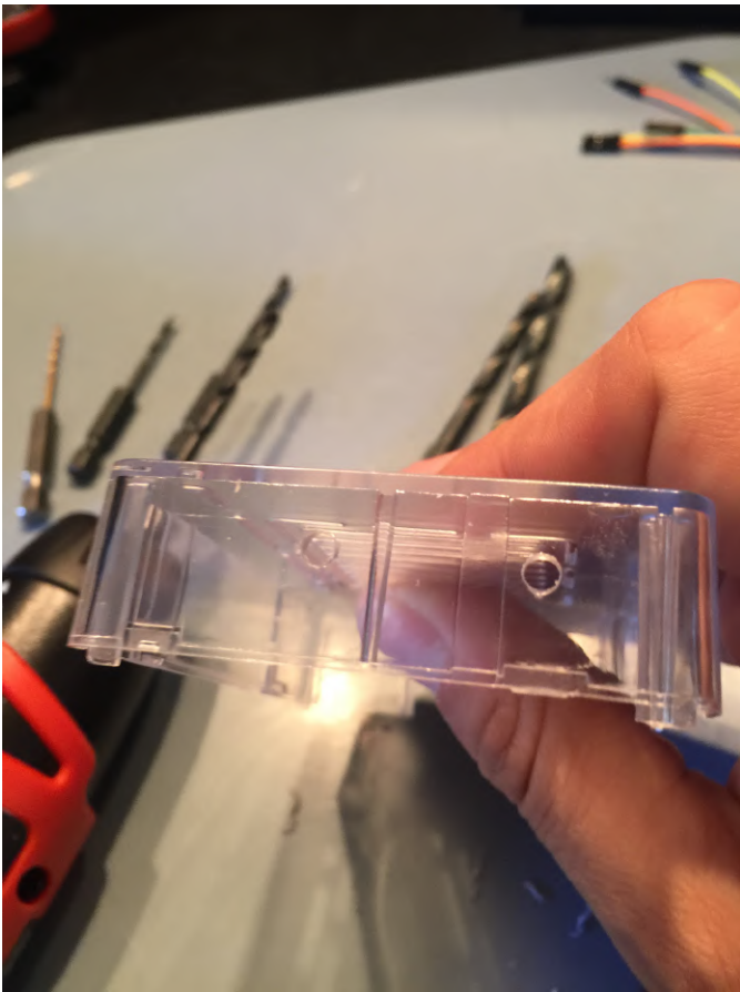
Figures 5 and 6 - Each run-through with a bigger drill bit creates a slightly larger hole
