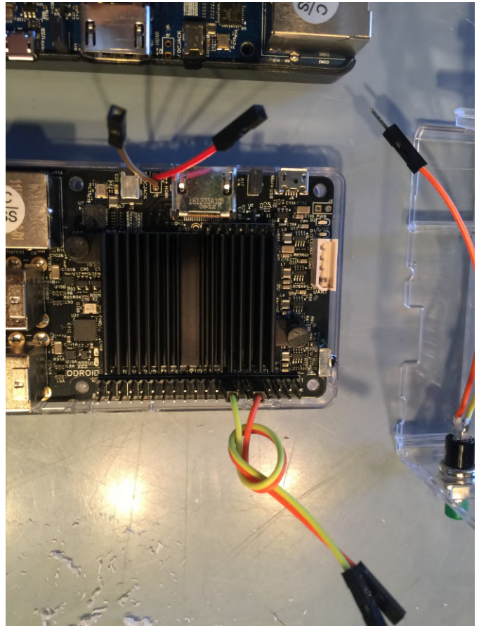
Figure 7 - Place one jumper on pin 9, GROUND, of the 40-pin GPIO header
