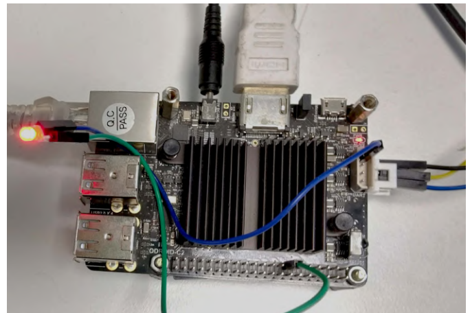
Figure 3 - Led Connection on OdroidC2 Board
