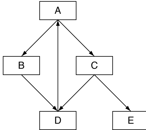
Figure 5: An asynchronous cyclic module graph
