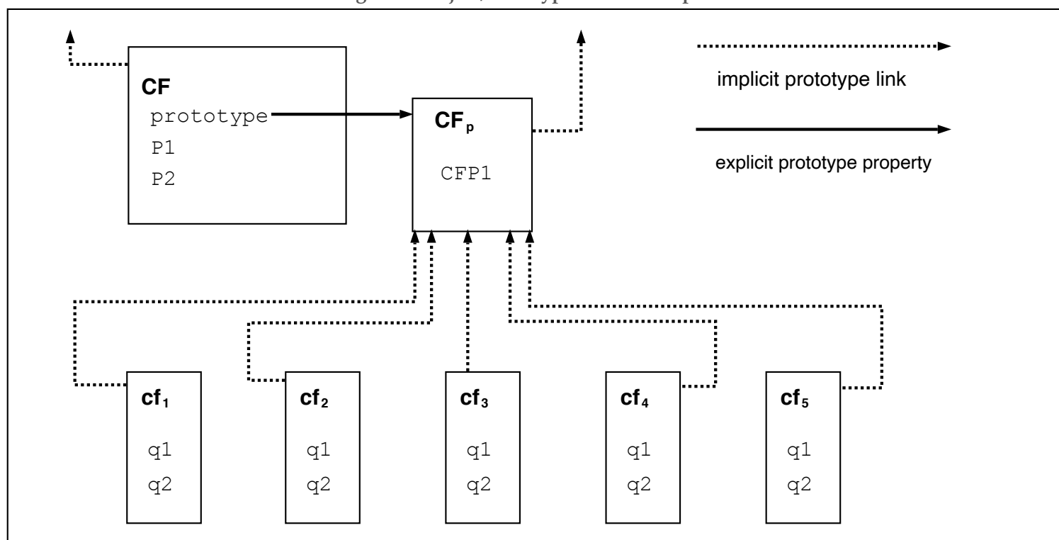
Figure 1: Object/Prototype Relationships
