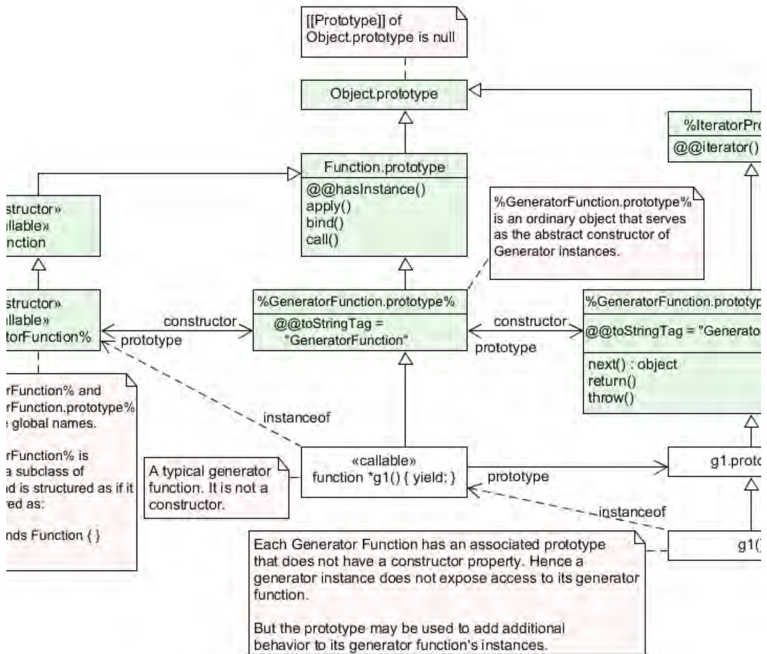
Figure 6 (Informative): Generator Objects Relationships
