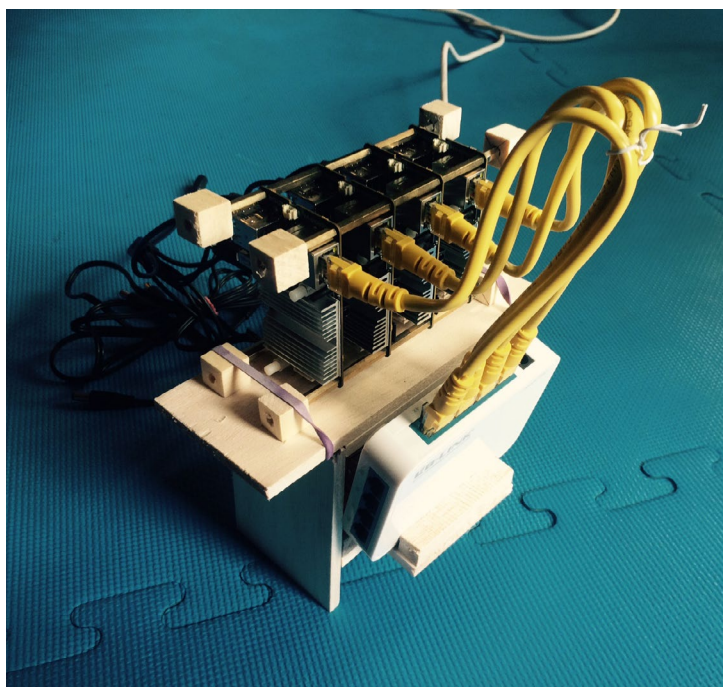
My Home Compute Cluster using 4 X ODROID-U3
