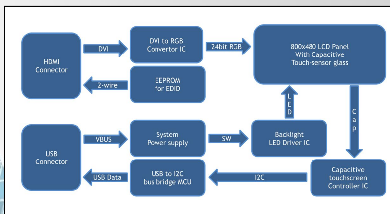
Multi-touch screen block diagram
