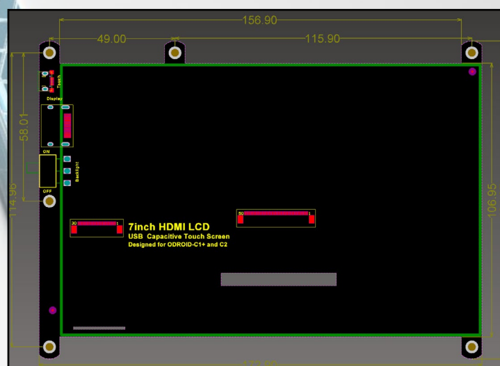
Rear side view and physical dimensions
