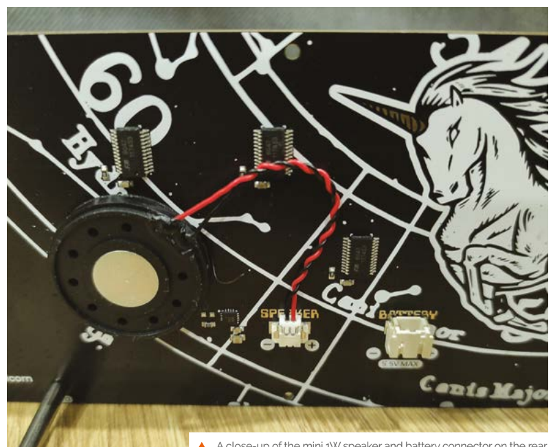
▲ A close-up of the mini 1W speaker and battery connector on the rear
