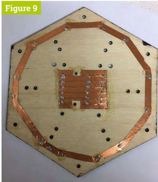
▲ Figure 9 Grounding copper foil
