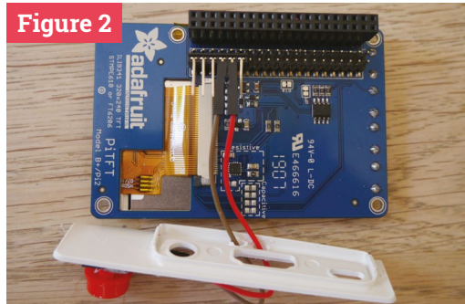
▲ Figure 2 There isn't enough room to attach jumper wires to the pins on the screen. If you don't want to solder on wires, use a 90-degree header
