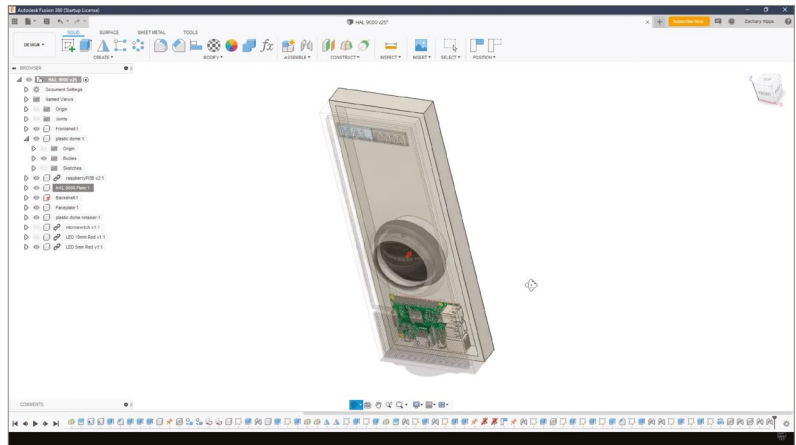
▲ Designing the case in Fusion 360, ready for 3D printing
