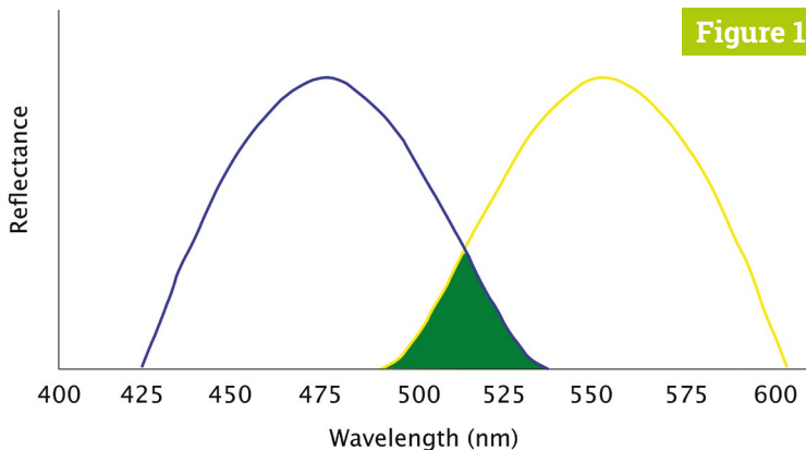
▲ Figure 1 Blue and yellow paint mixed gives green
