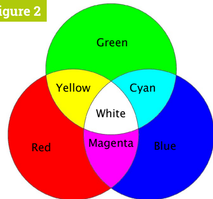
▲ Figure 2 RGB additive system using light
