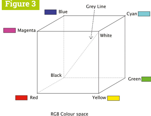
▲ Figure 3 RGB additive system using light
